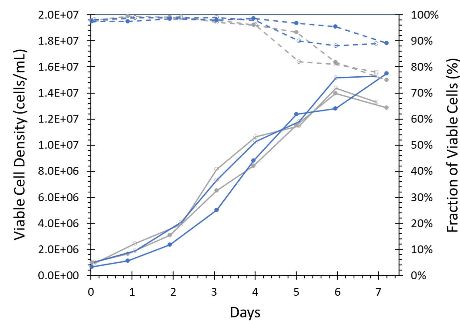
Figure 5: Viable cell densities and viabilities during Appliflex ST (silver) and miniBio bioreactor runs using an open hole sparger. Open and closed markers indicate duplicate experiments
