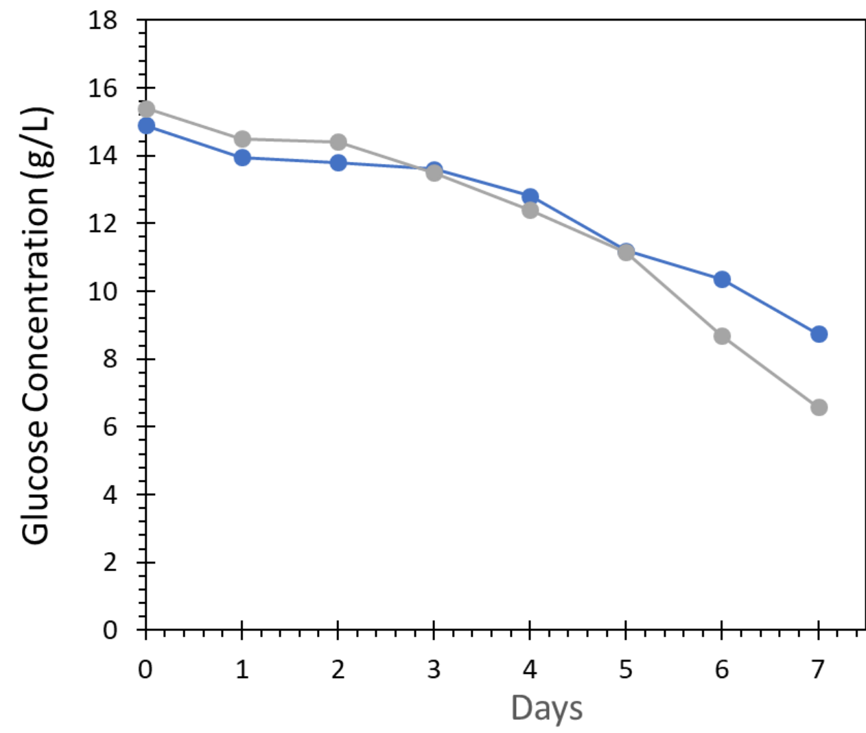
Figure 4: Glucose concentrations during Appliflex ST (silver) and miniBio (blue) bioreactor runs using a porous sparger.
