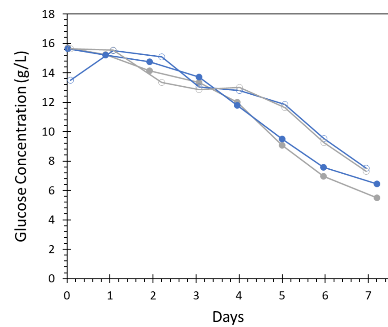
Figure 6: Glucose concentrations during Appliflex ST (silver) and miniBio bioreactor runs using an open hole sparger. Open and closed markers indicate duplicate experiments
