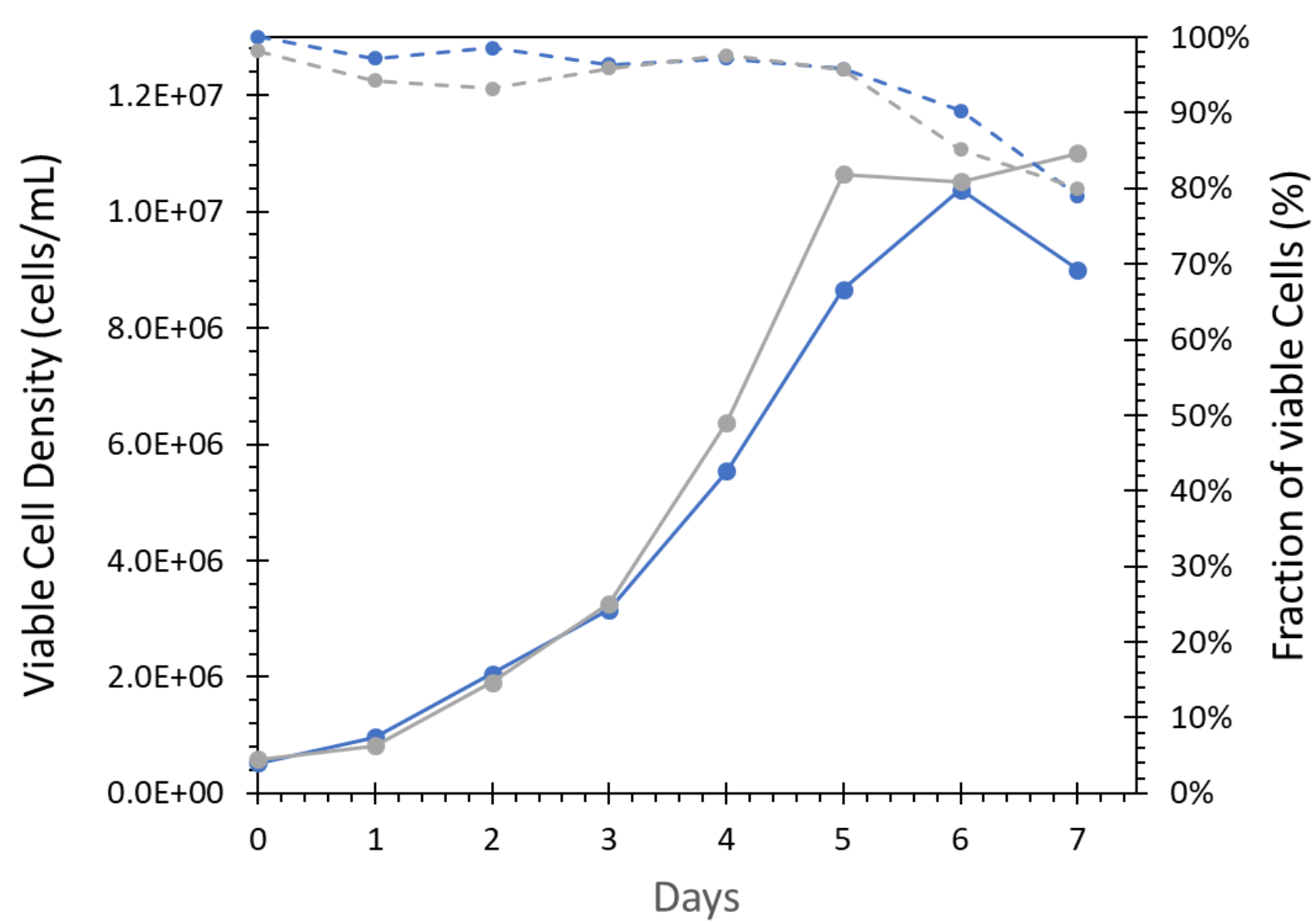
Figure 3: Viable cell densities and viabilities during Appliflex ST (silver) and miniBio (blue) bioreactor runs using a porous sparger.
